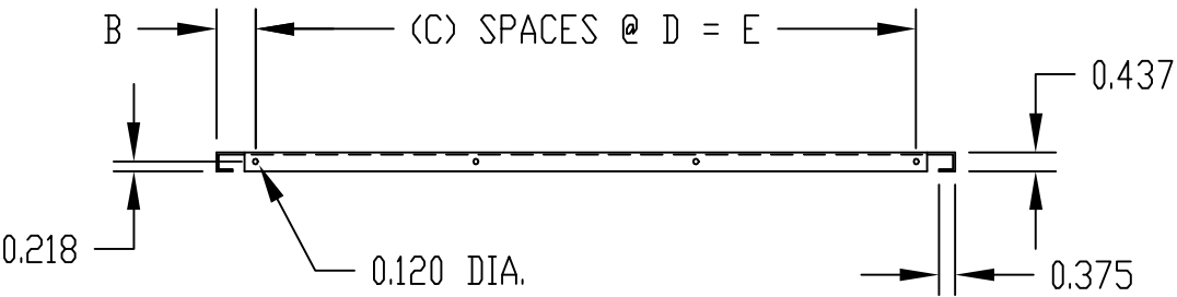
VENTILATED TOP OR BOTTOM COVER TBC-14262 & TBC-14263
