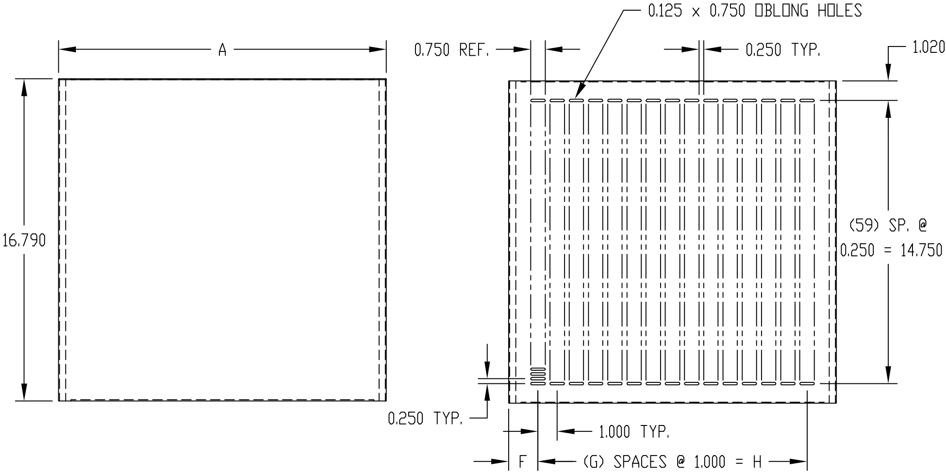
SOLID TOP OR BOTTOM COVER TBC-14252 & TBC-14253
