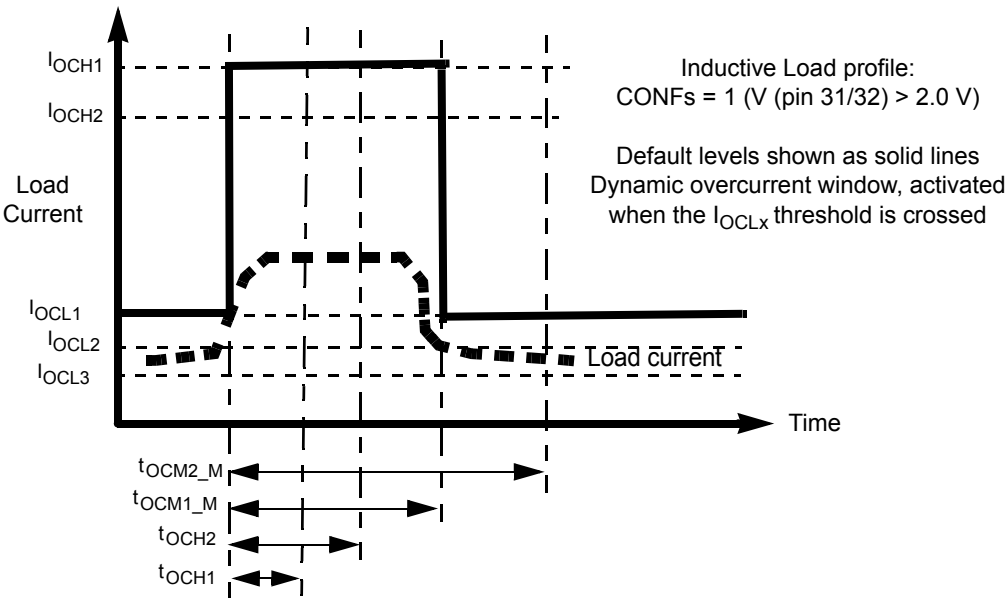
Figure 6. Overcurrent Protection Profile for Applications with Inductive Loads (DC motors, solenoids)
