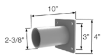
T02 - 2-3/8" tenon wall mount
