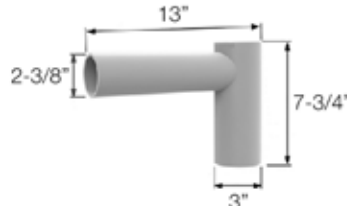
T03 - 2-3/8" tenon to slipfitter adapter
