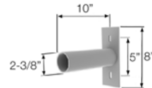
T01 - 2-3/8" tenon side of square pole mount
