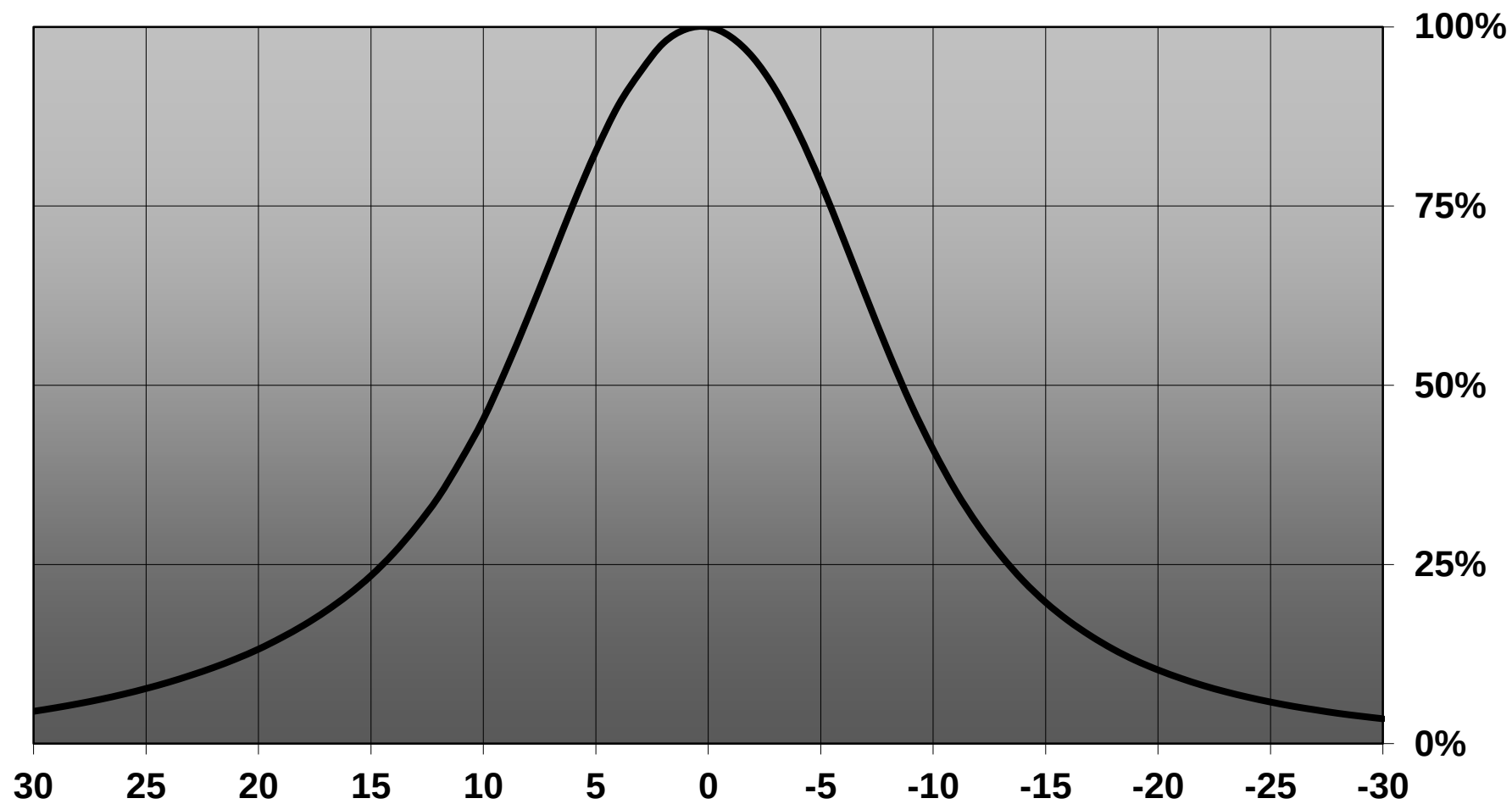
Relative intensity of C13234_SATU-S_(SSL80)
