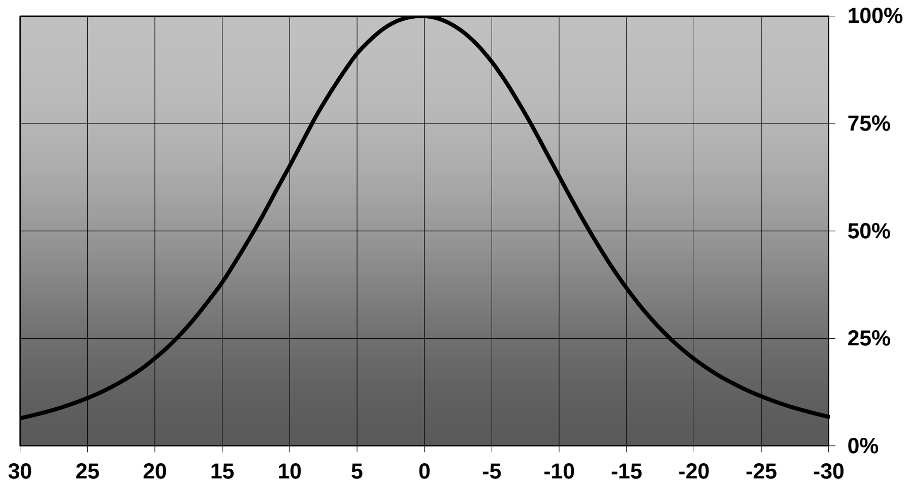
Relative intensity of C13234_SATU-S_(XP-G)
