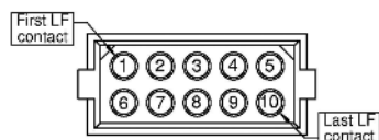
Female connectors ( shown looking onto mating face )
