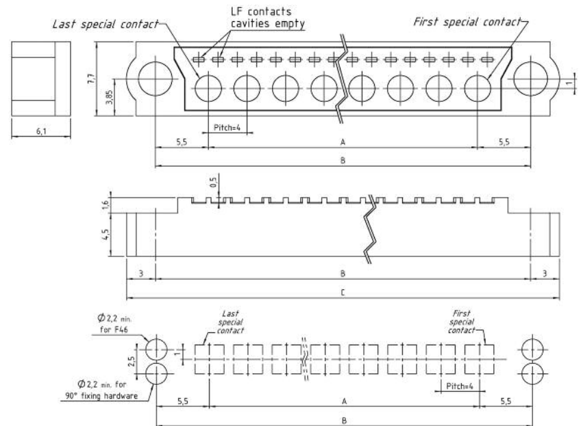
HP 30-3400-xx PCB lay-out
