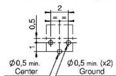
HF 30-1400-xx PCB lay-out
