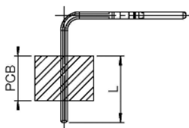
90° on PCB
