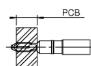
Pressfit Straight on PCB
