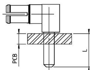
90° on PCB
