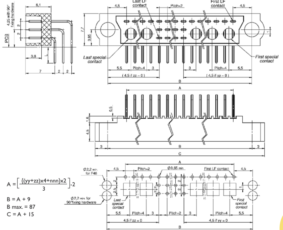
HP 30-3400-xx PCB lay-out
