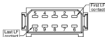
Male connectors ( shown looking onto mating face )
