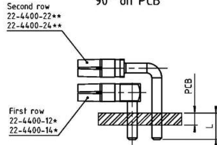
90° on PCB
