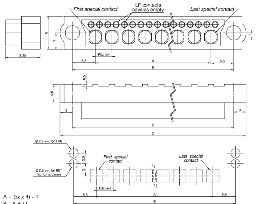
HP 30-4400-xx PCB lay-out
