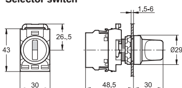
Selector switch
