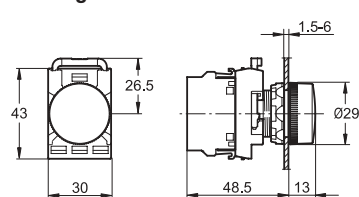
Pilot light
