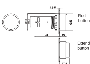
Pushbutton
