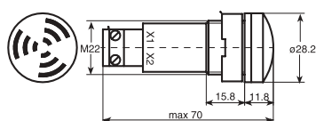
Buzzer
