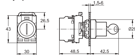
Key-operated selector switch
