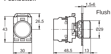
Pushbutton
