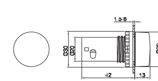
Pilot light
