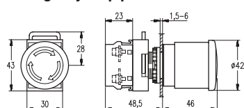
Emergency stop pushbutton
