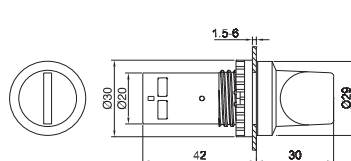
Selector switch
