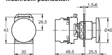
Mushroom pushbutton
