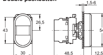
Double pushbutton
