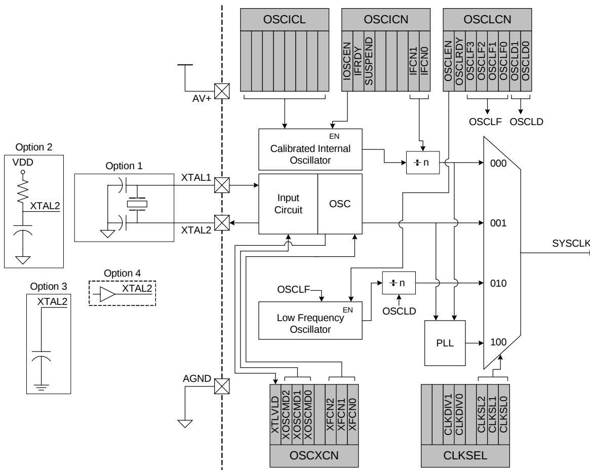
Figure 16.1. Oscillator Diagram
