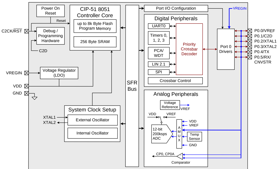
Figure 1.2. C8051F52xA/F52x-C Block Diagram
