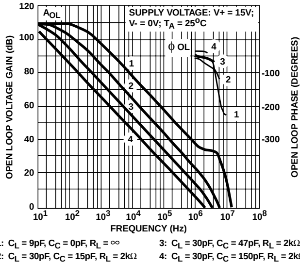
FIGURE 13. OPEN LOOP VOLTAGE GAIN AND PHASE SHIFT vs FREQUENCY
