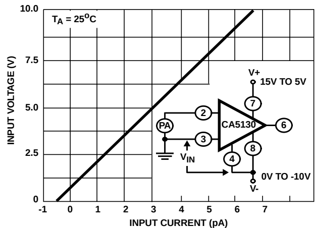
FIGURE 24. INPUT CURRENT vs COMMON MODE VOLTAGE
