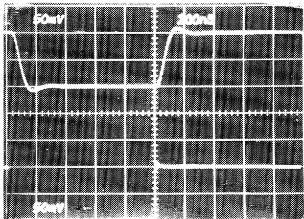
FIGURE 3A. SMALL SIGNAL RESPONSE (50mV/DIV., 200ns/DIV.)
