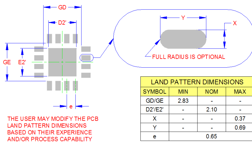
Figure 6.3 16-Pin QFN 4mm x 4mm PCB Footprint
