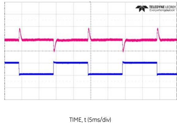
Figure 8. Transient response 12V DC output load step 50 – 100A, V IN = -48V DC .
