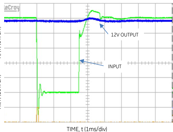
Figure 12. Ride through: full load V IN = -48V DC
