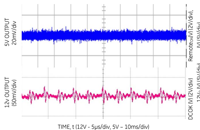
Figure 5. 12V output ripple and noise (Vin: -48V DC , full load).
