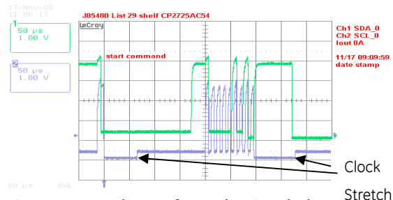
Figure 1. Example waveforms showing clock stretch
