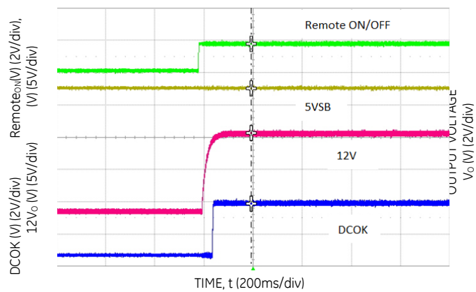
Figure 3. Start-up Using Remote On/OFF (Vin: -48V DC , full load)
