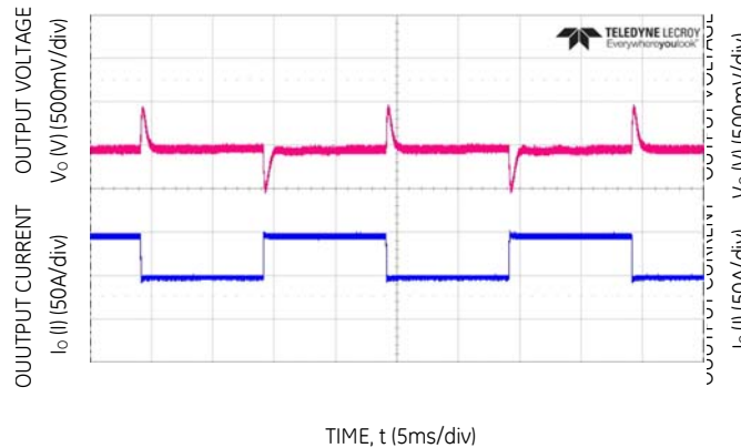
Figure 7. Transient response 12V DC output load step 10 – 60A, V IN = -48V DC .
