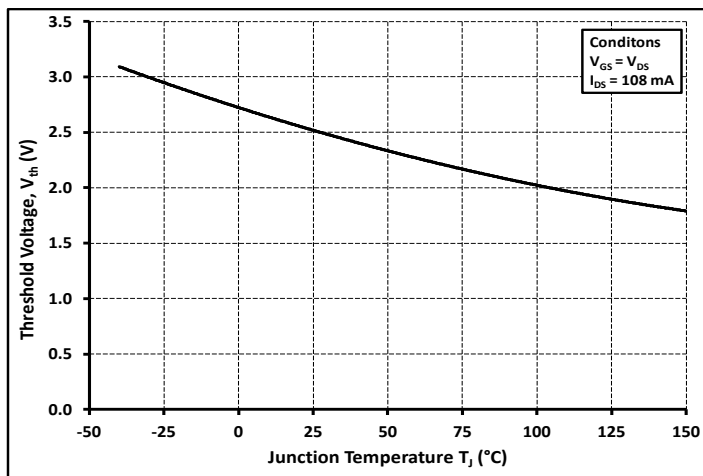
Figure 7. Threshold Voltage vs. Temperature
