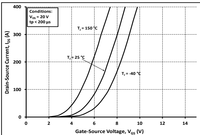
Figure 8. Transfer Characteristic for Various Junction Temperatures
