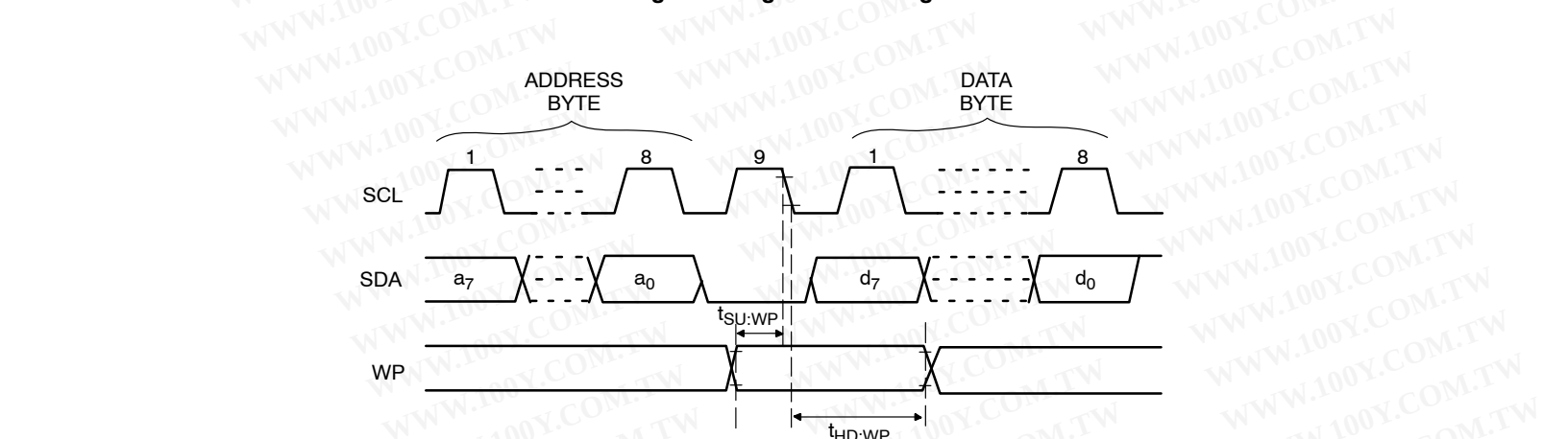
Figure 9. WP Timing
