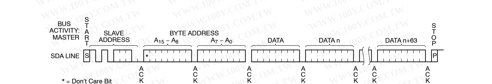
Figure 8. Page Write Timing
