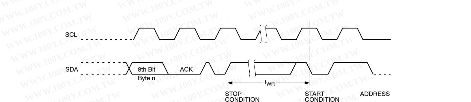
Figure 7. Write Cycle Timing
