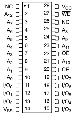
SOIC Package (J, K, W, X)
