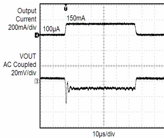
Load Transient Response (0.1mA to 150mA)
