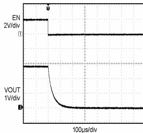
Enable Turn-Off (150mA Load)
