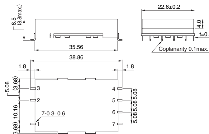
CC10-R-E (SMD TYPE)
