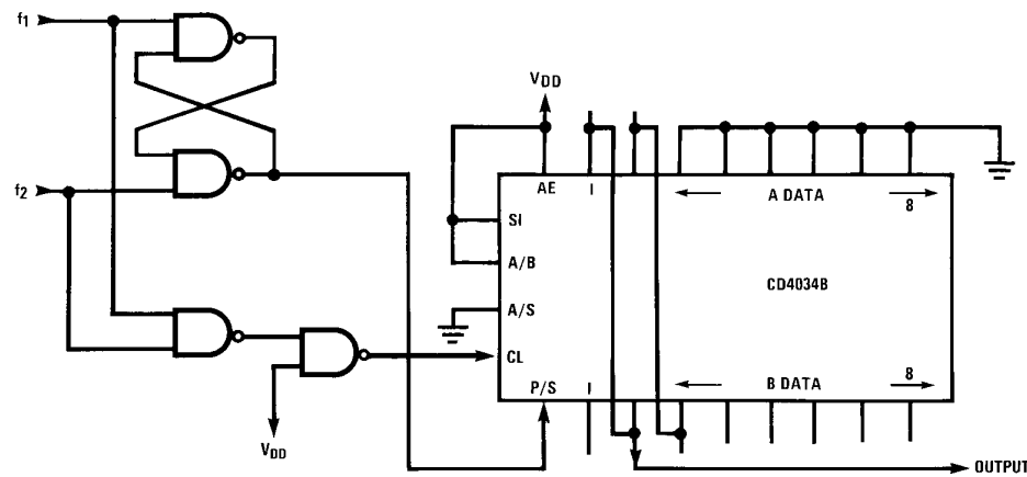
Frequency and Phase Comparator
