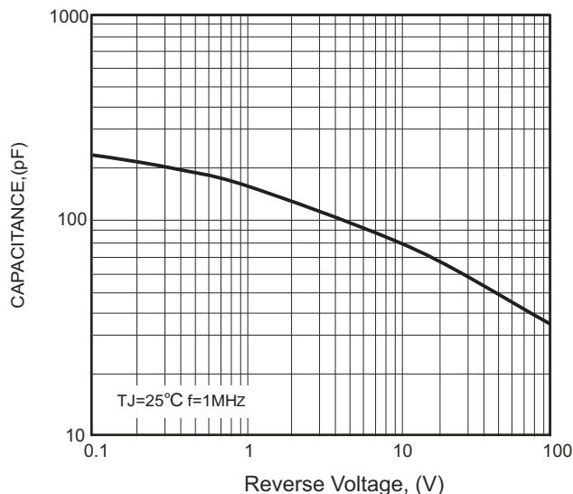
FIG.4-TYPICAL JUNCTION CAPACITANCE
