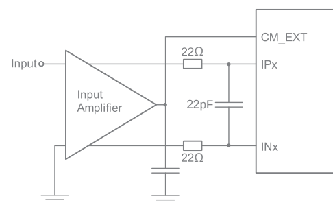
Figure 3. DC-Coupled Input
