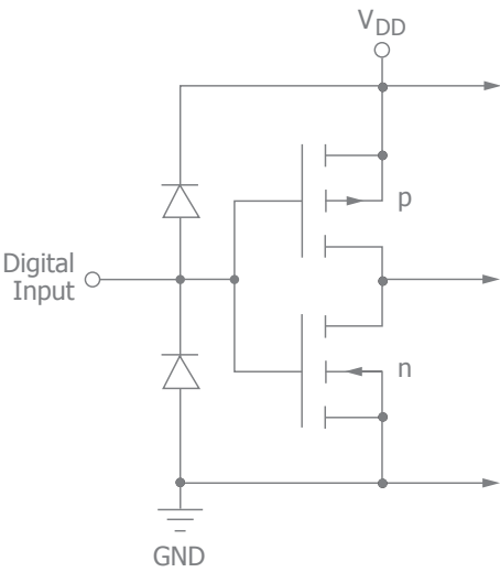
Figure 3. Equivalent Digital Input Circuit
