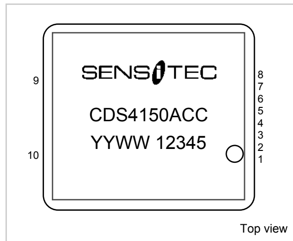
Fig. 5: Pinning of CDS4150ACC.
