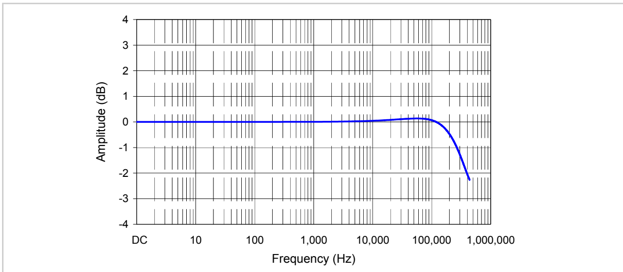
Fig. 11: Typical frequency response by using a RC-filter with the parameters R_f = 1.0 \text{ k}\Omega and C_f = 39 \text{ nF} .
