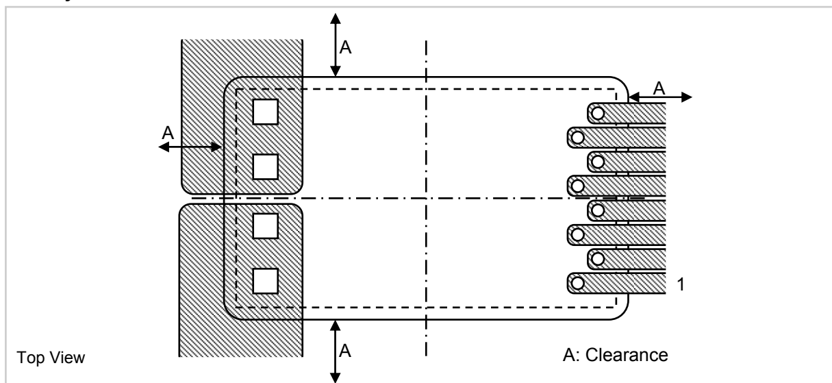
Fig. 9: Recommended PCB layout for the CDS4150 sensor (schematic).
