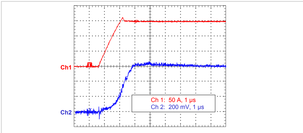
Fig. 10: Typical output characteristic due to a current jump from 0 to I_{PN} . Input di/dt \approx 120 \text{ A}/\mu\text{s} . An RC-filter with the parameters R_f = 1.0 \text{ k}\Omega and C_f = 39 \text{ nF} is used.
