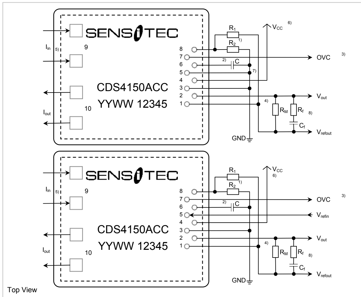
Fig. 7: Top : Example of how to use the internal reference voltage (pin 5, V_{refin} is routed on ground). Bottom : Circuit with external reference voltage at pin 5, V_{refin} .
