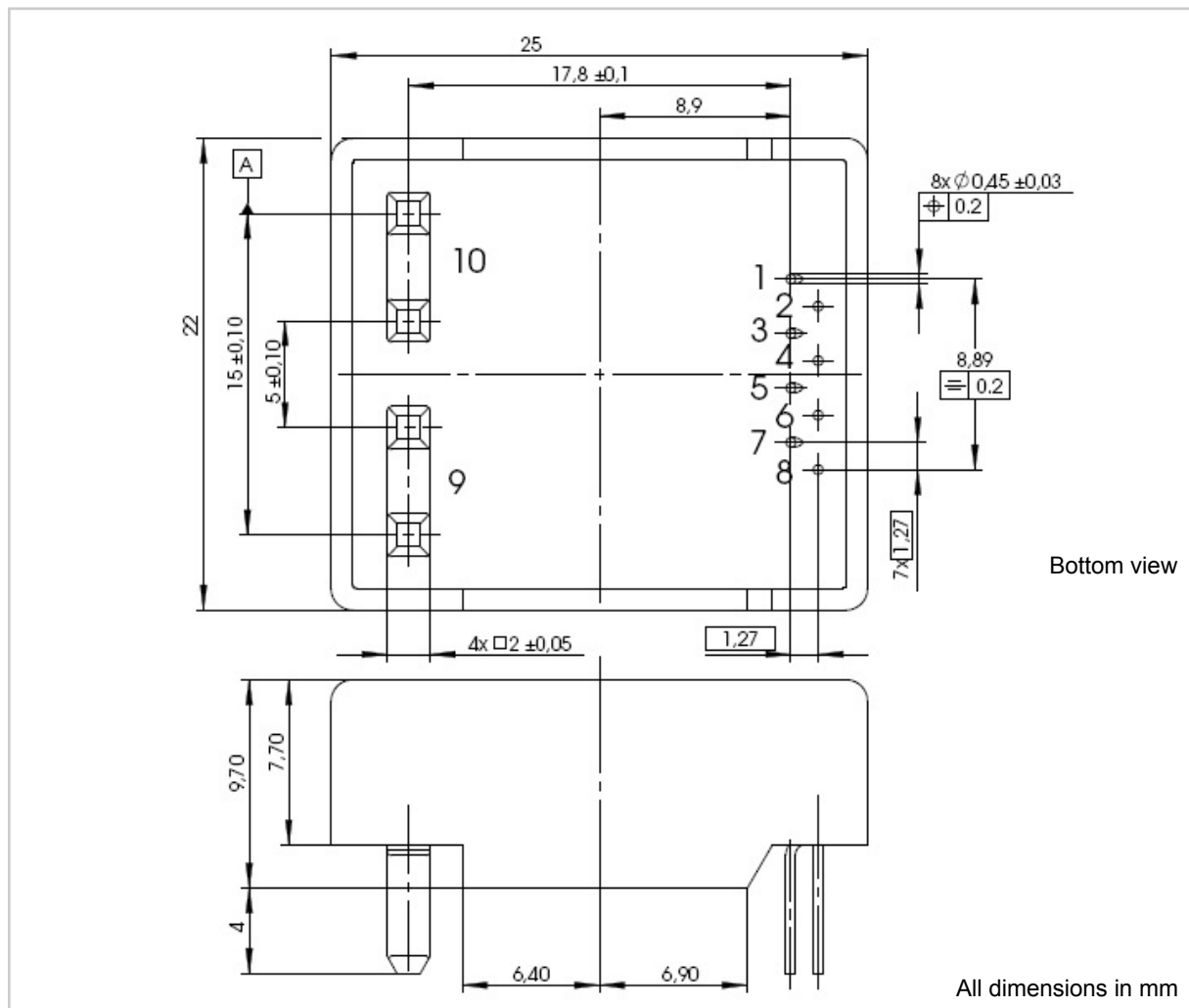
Fig. 6: Package outline of THT-housing. Tolerance \pm 0.2\text{ mm} unless otherwise specified.
