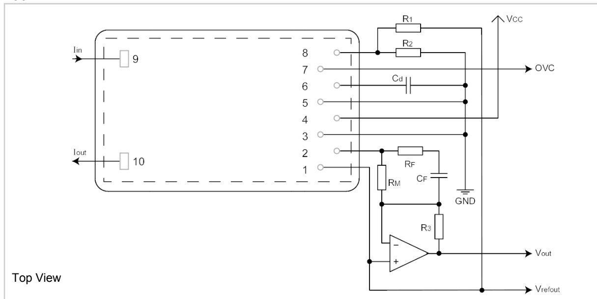
Fig. 8: Example of how to use an operational amplifier to adjust the output signal to an A/D converter. With R_M = 300 \Omega and R_3 = 410 \Omega , the output signal is amplified to a full scale output of 4.92 V.
