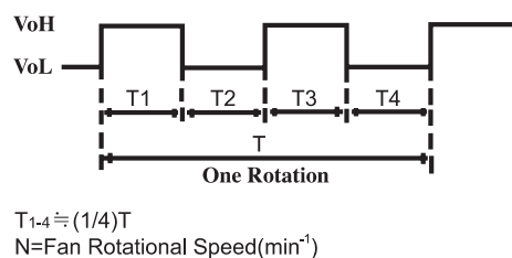
Figure 4 Output Waveform
