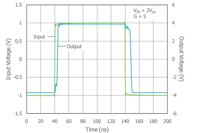
Figure 7. Overdrive Recovery
