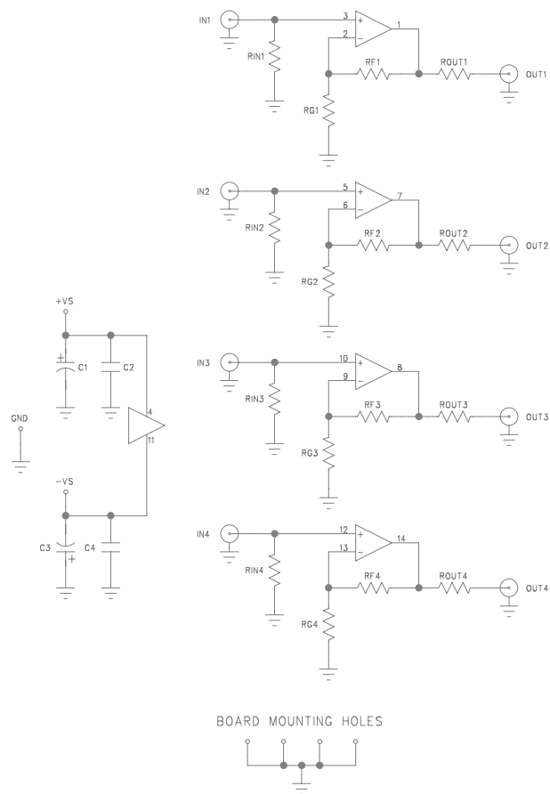
Figure 18. CEB018 &amp; CEB017 Schematic
