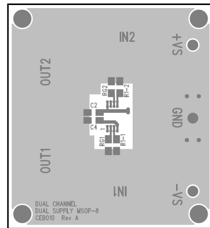
Figure 11. CEB010 Top View
