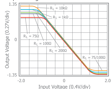
Output Swing vs. Load
