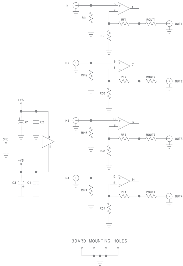
Figure 14. CEB018 Schematic
