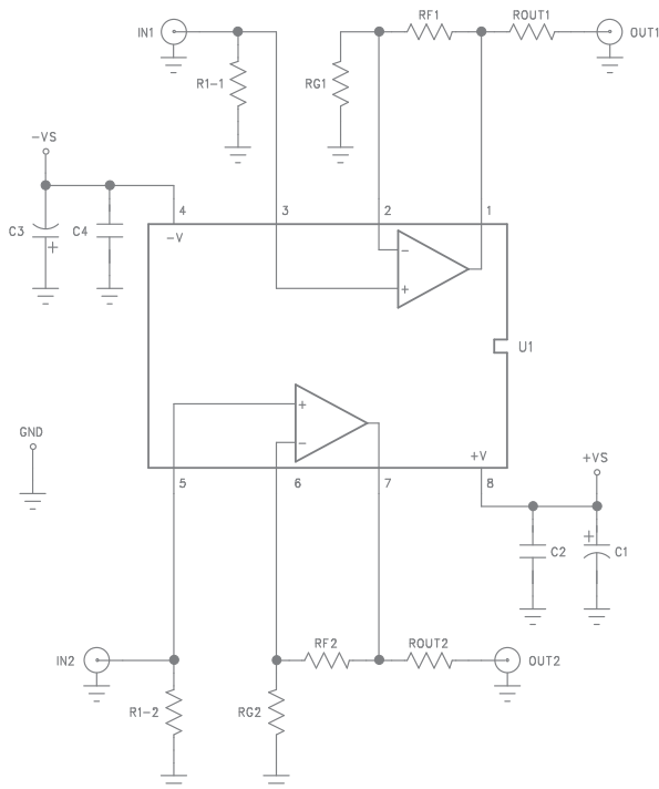
Figure 11. CEB006 Schematic
