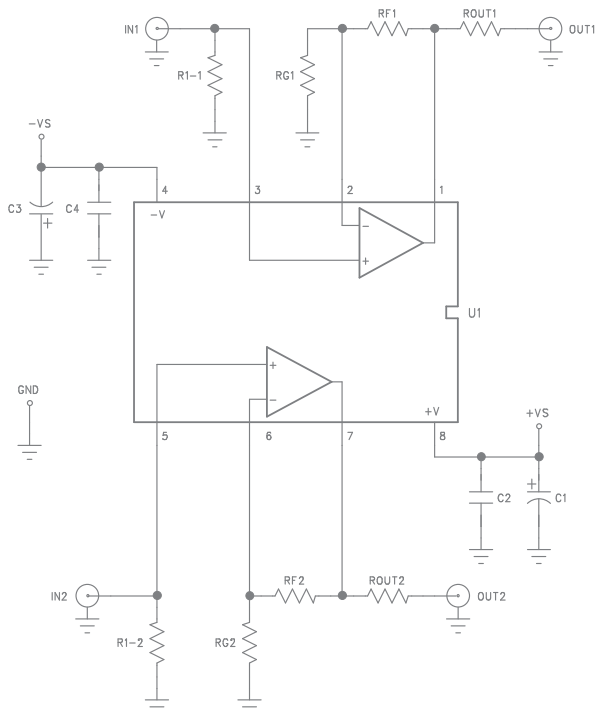
Figure 10. CEB006 Schematic
