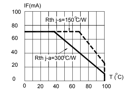
FIG.5 MAXIMUM FORWARD DC CURRENT VS AMBIENT TEMPERATURE (Tjmax=110°C)
