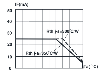
FIG.5 MAXIMUM FORWARD DC CURRENT VS AMBIENT TEMPERATURE ( T_{jmax}=110^{\circ}\text{C} )
