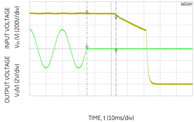
Figure 8. Typical Hold-up waveforms ( V_{IN} = 230V , 100% load).
