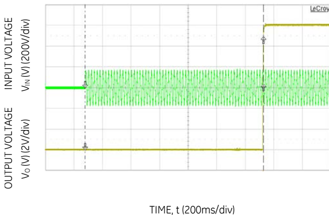
Figure 5. Typical Start-up ( V_{IN} = 115\text{Vac} ).
