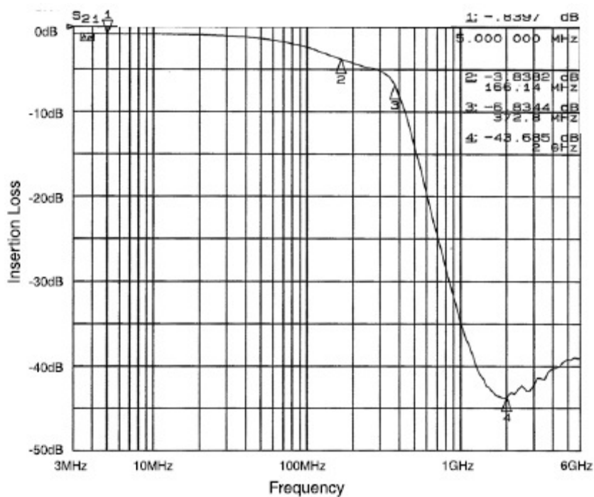
Figure 2. Filter 2 Insertion Loss (CM1460-04DE)
