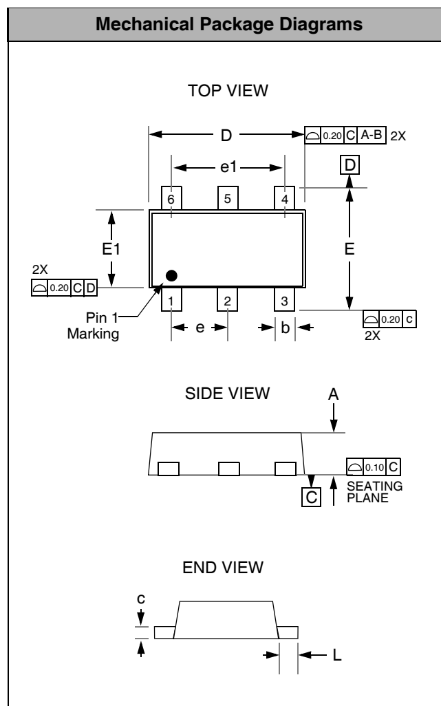
Package Dimensions for SOT-563.
