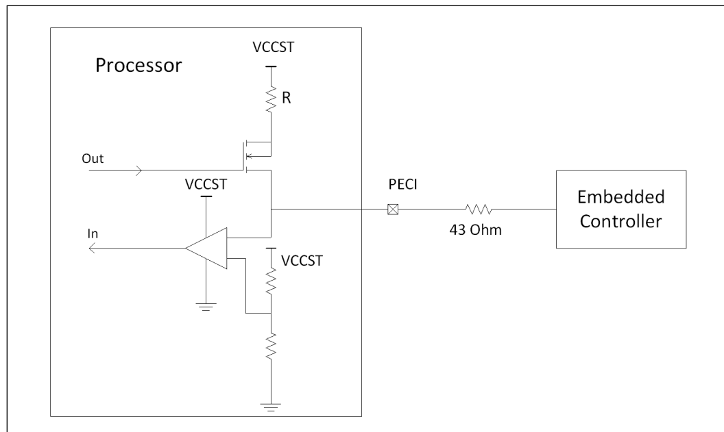
Figure 2-10. Example for PEI EC Connection
