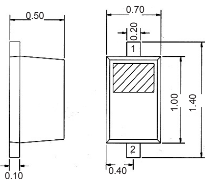
Pkg Dimensions (mm)
