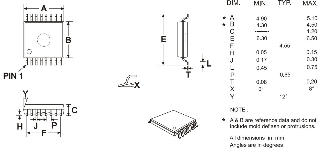
Figure 14 : 16-pin TSSOP Mechanical Outline: Order as part no. CMX602BE4
