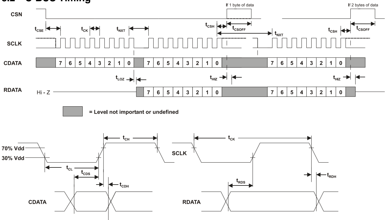
Figure 19 C-BUS Timing
