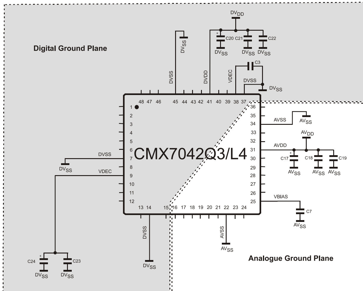
Figure 5 CMX7042 Power Supply Connections and De-coupling
