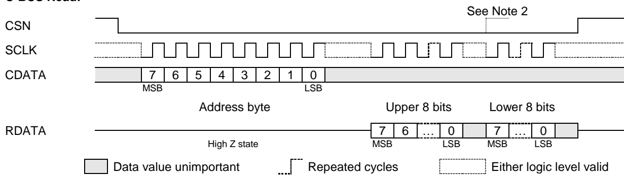
Figure 6 C-BUS Transactions
