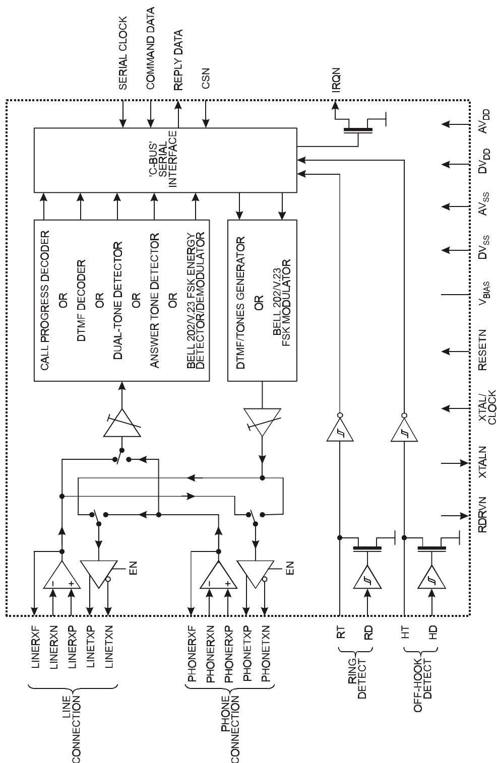
Figure 1 Block Diagram
