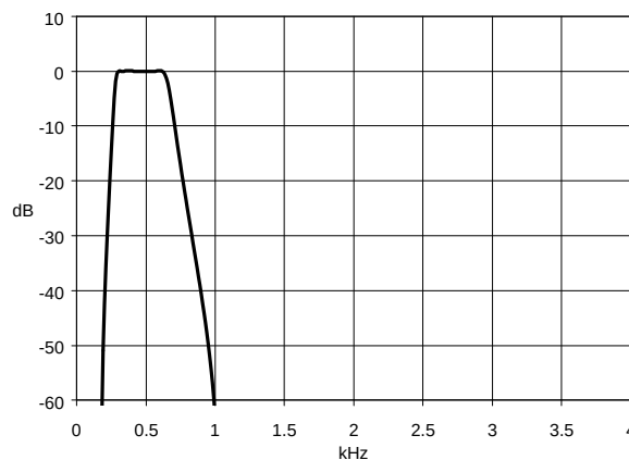
Figure 5a Response of the Call Progress Filter
