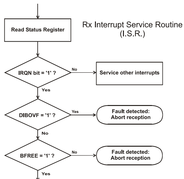
Figure 15 Receive Process
