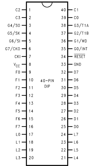
Top View
