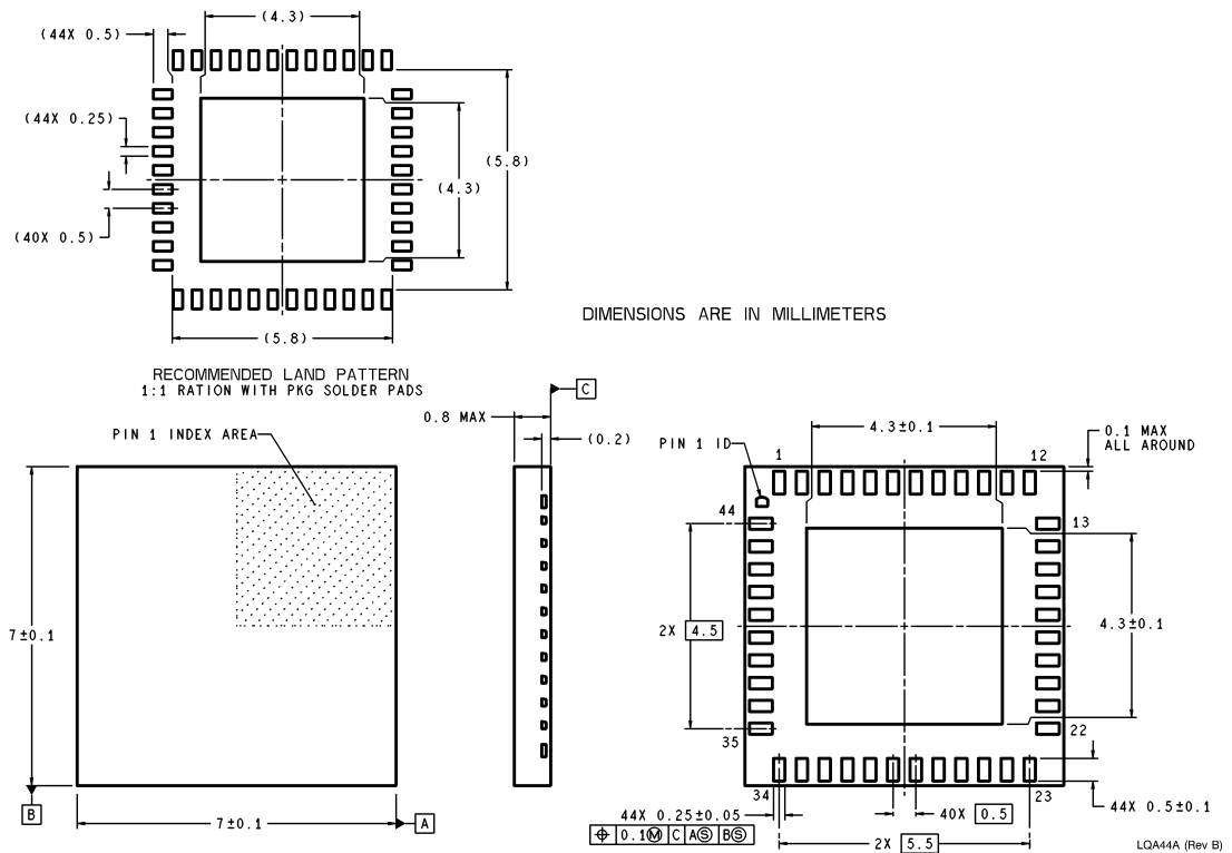
Chip Scale Package CSP Order Number COP8SGR7HLQ8 NS Package Number LQA44A
