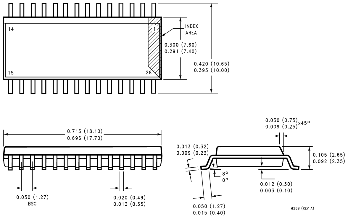
Molded SO Wide Body Package (WM) Order Number COP8SGx528Mx, NS Package Number M28B
