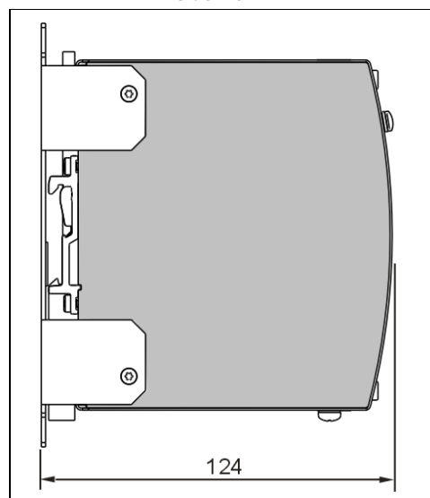
Fig. 24-6 Wall/panel mounting, side view
