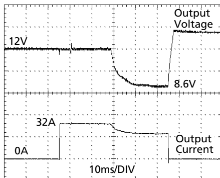
Fig. 25-1 32 A Resistive peak load (2x the nominal current) for 50ms, typ.
