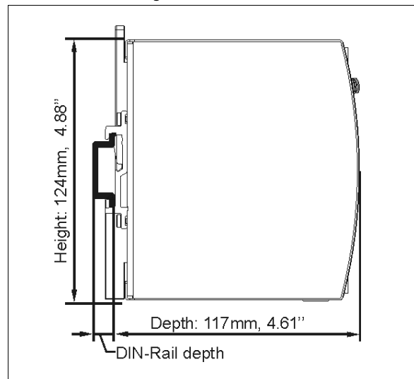
Fig. 23-2 Side view
