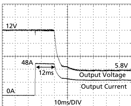
Fig. 25-3 48 A Resistive peak load (3x the nominal current) for 12ms, typ.
