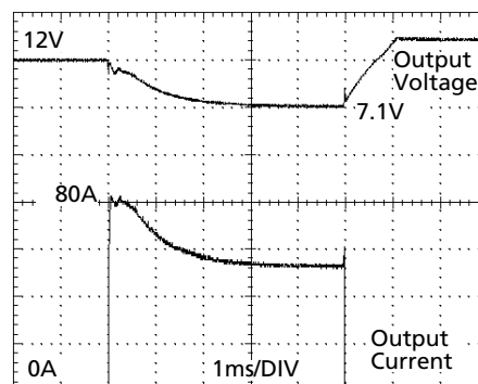
Fig. 25-2 80 A Resistive peak load (5x the nominal current) for 5ms, typ.
