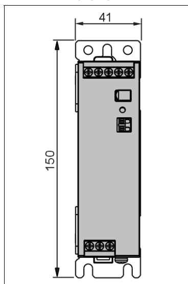
Fig. 24-4 Wall/panel mounting, front view
