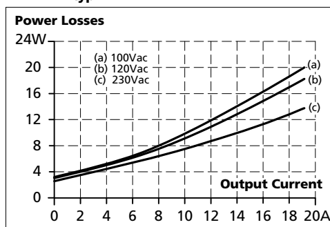
Fig. 10-2 Losses vs. output current at 12V, typ.
