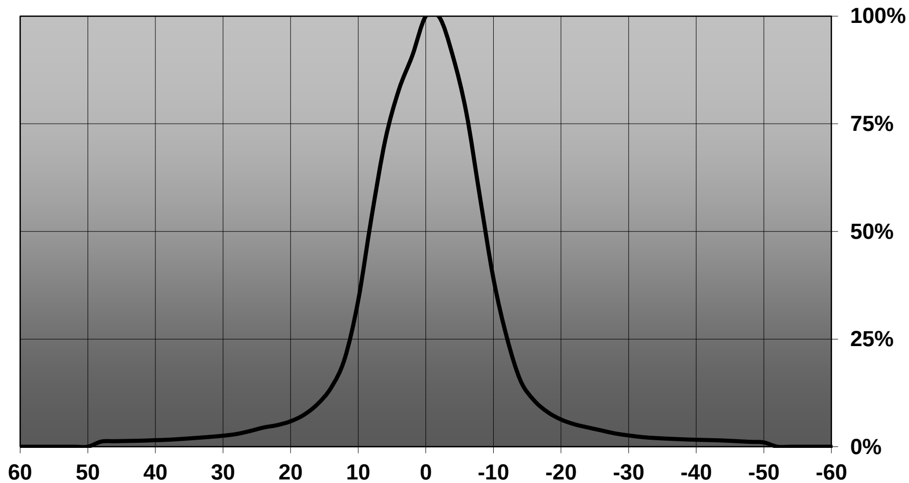
Relative intensity of CP13072_Irene-IR-16_(SFH4725S)
