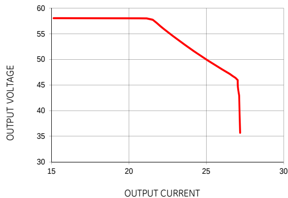
Figure 3. 54V DC output: Power limit, Current limit and shutdown profile at V_{IN} = 90V_{AC} .
