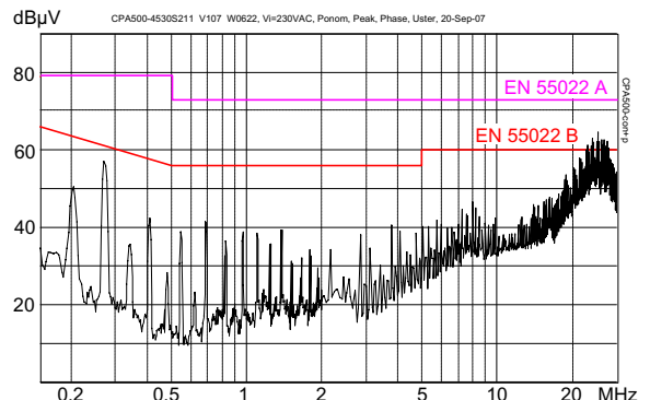
Fig. 15 CPA500-4530: Typical disturbance voltage at line input accord. to EN 55011/22, measured at V_{i \text{ nom}} and P_{o \text{ nom-}} .
