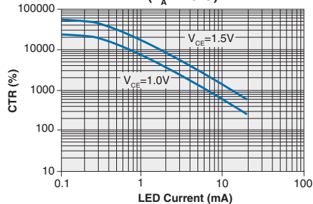
CTR vs. LED Current ( I_F ) ( T_A = 25^\circ\text{C} )
