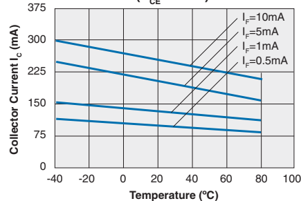
Collector Current vs. Temperature ( V_{CE} = 1.2\text{V} )
