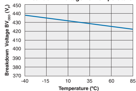
Breakdown Voltage vs. Temperature
