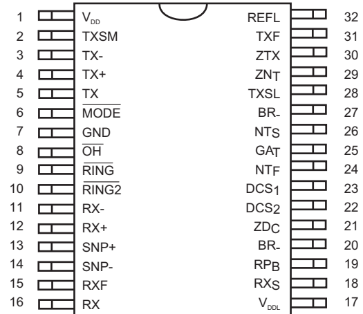
Figure 1. Pinout
