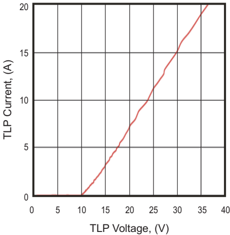
Fig.6 - Positive TLP IV Curve
