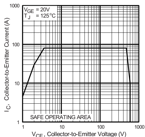
Fig. 12 - Turn-Off SOA
