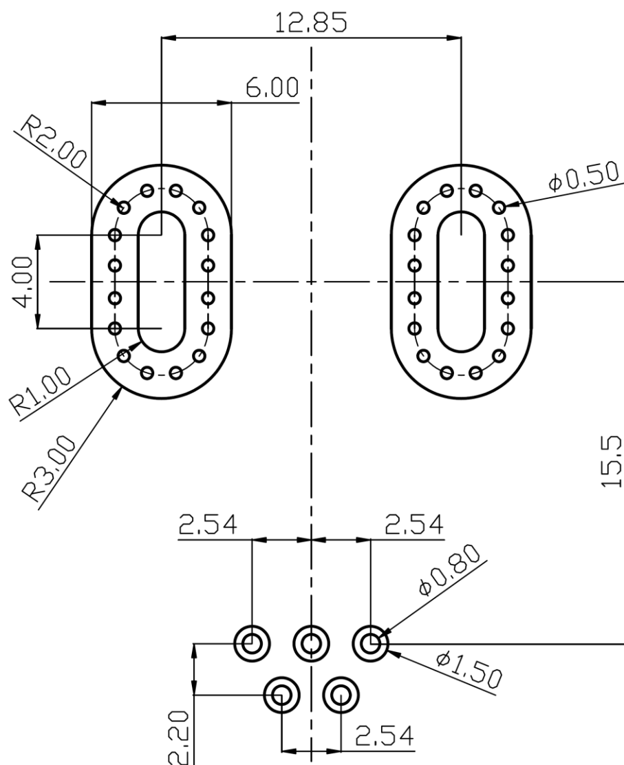
Figure 11. Package outline
