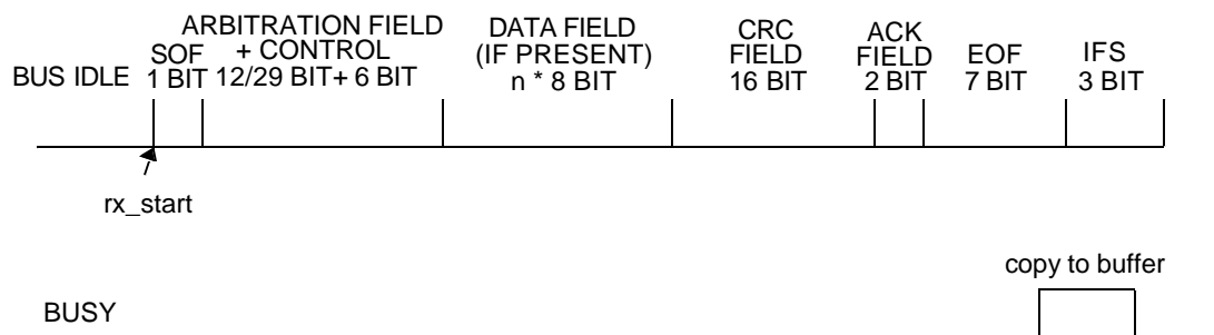
Figure 61. Receive Timing
