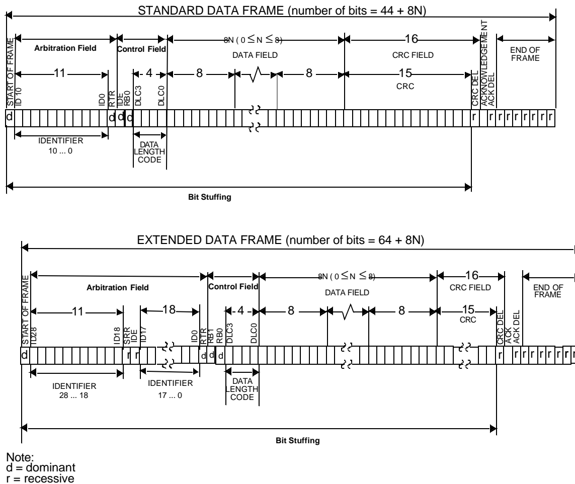
Figure 46. CAN Data Frame (standard and extended)
