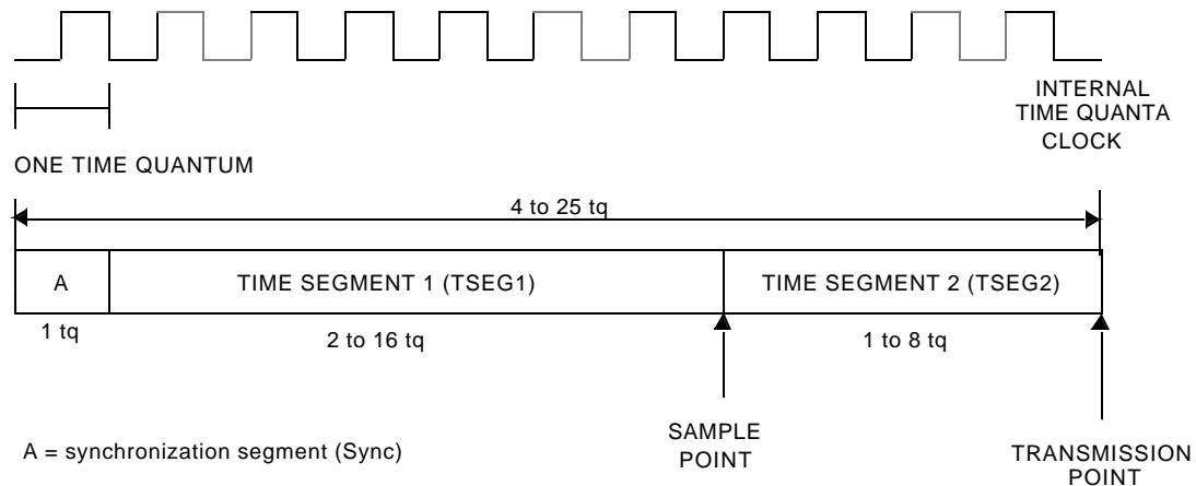
Figure 52. Bit Timing
