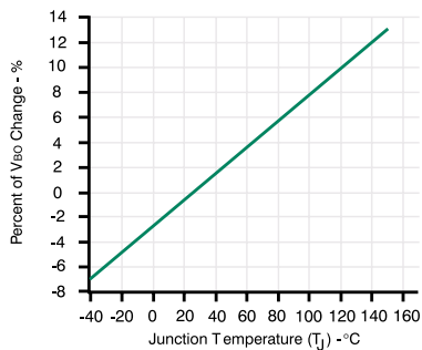
TYPICAL V_{BO} CHANGE vs JUNCTION TEMPERATURE
