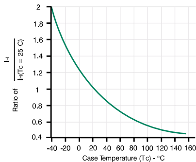
TYPICAL DC HOLDING CURRENT vs CASE TEMPERATURE
