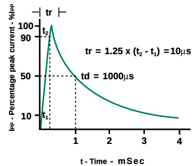
PULSE WAVE FORM (10/10000 \mu S)
